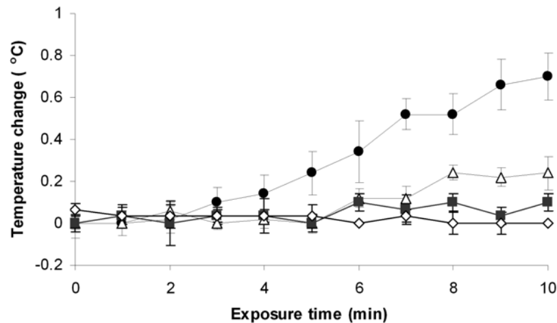
Figure 2. US-induced temperature changes at the monolayer surface of the culture flask. I_{SATA} levels were (◊) 0 mW/cm 2 control, (■) 130 mW/cm 2 , (△) 480 mW/cm 2 , (●) 1770 mW/cm 2 . The ambient water bath temperature was 37.4°C. Results are presented as mean ±SE.
