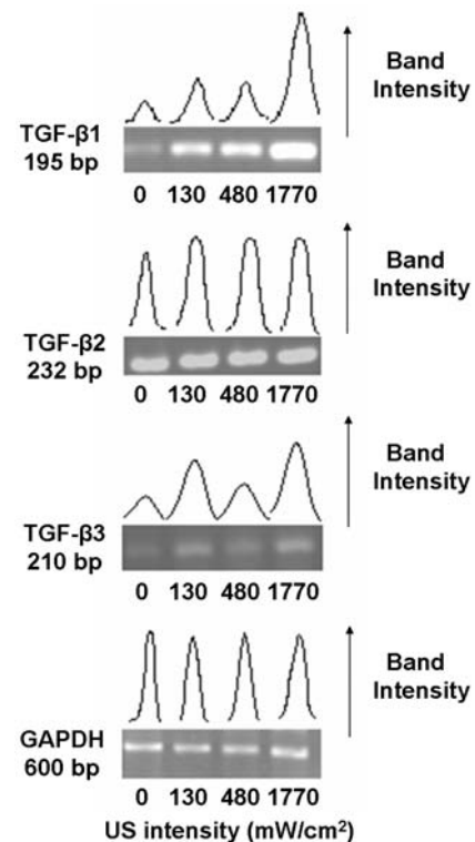
Figure 1. Representative agarose electrophoresis gels of the RT-PCR products of the TGF- \beta genes in MG63 cells exposed to different intensities of US (0, 130, 480, 1770 mW/cm 2 ). Image analysis of the resulting band intensities is also shown, including that of the housekeeping gene, GAPDH, in each cDNA sample.
